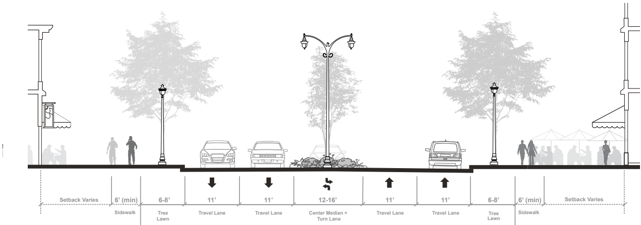
Saturn Road - Road Diet Street Section
